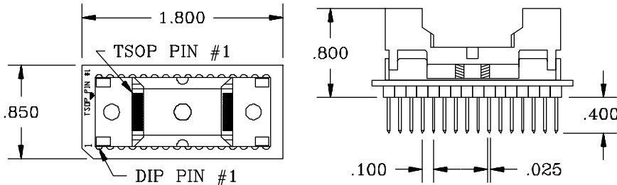
All Dimensions in Inches. (Assembly Drawing: F2119)
